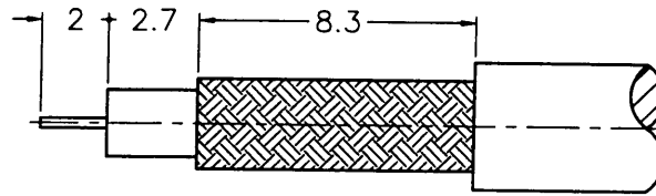
RECOMMENDED CABLE STRIPPING DIM'S (建議剝線尺寸)
